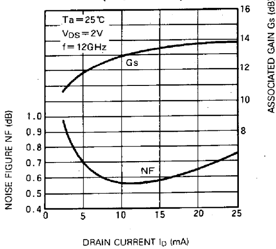
NF & G_s vs. I_D (f=12GHz) (MGF4918D)
